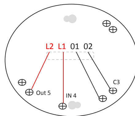
SMOKE DETECTOR BASE
