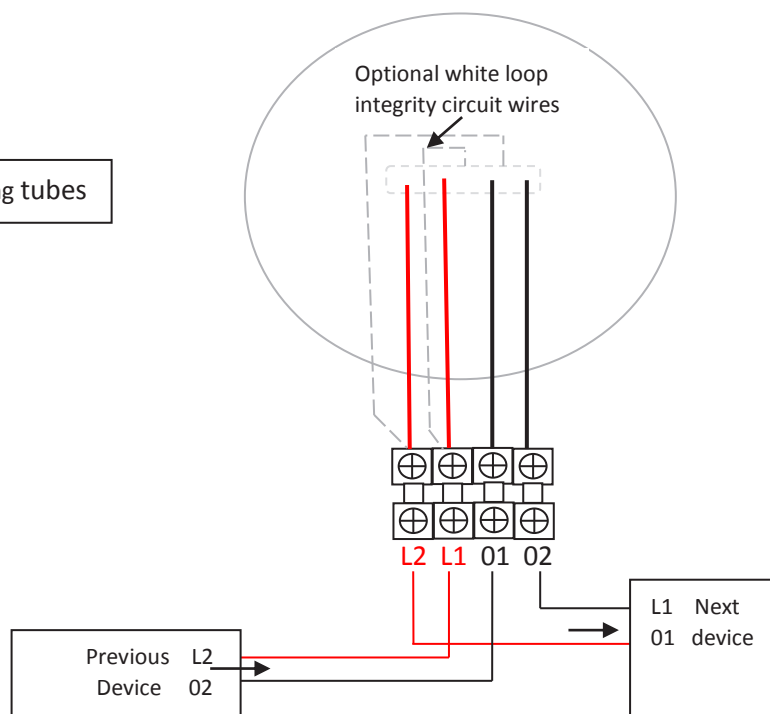
CEILING DISK A Diagram 1
